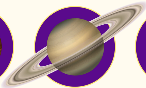
Saturn
