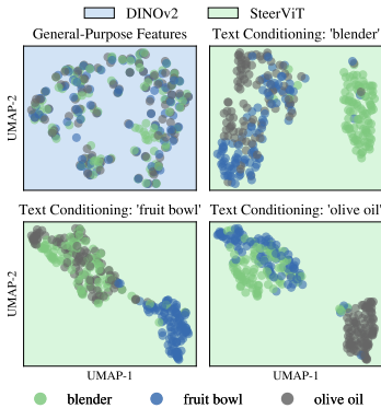
(a) Feature distribution across three object types in the “kitchen” scene.
