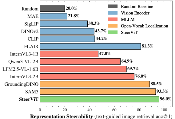
(b) Non-salient object retrieval performance on CORE across model families.
