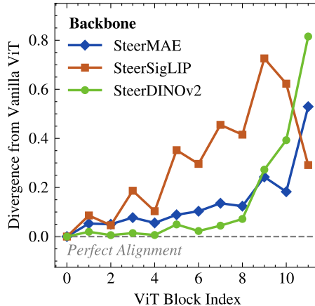
Fig. 14: Cosine divergence between SteerViT and base ViT intermediate features. Text-conditioning progressively steers internal features across layers.
