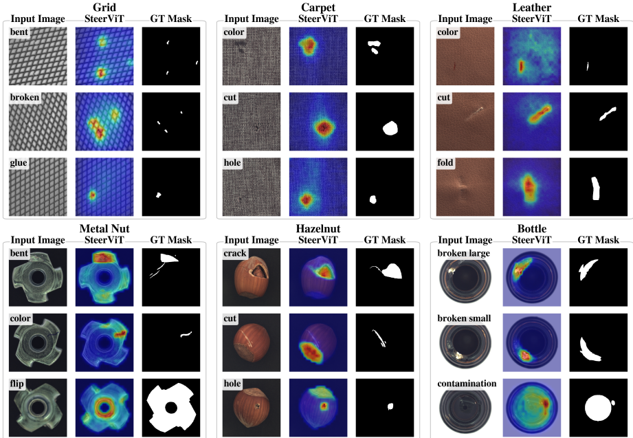
Fig. 16: Anomaly segmentation heatmaps predicted by SteerViT. We use the linear classification head optimized for patch-wise referential segmentation. Despite the stark task and domain gap, performance is especially good on texture-based classes (top) but also allows SteerViT to highlight small defects in objects (bottom).
