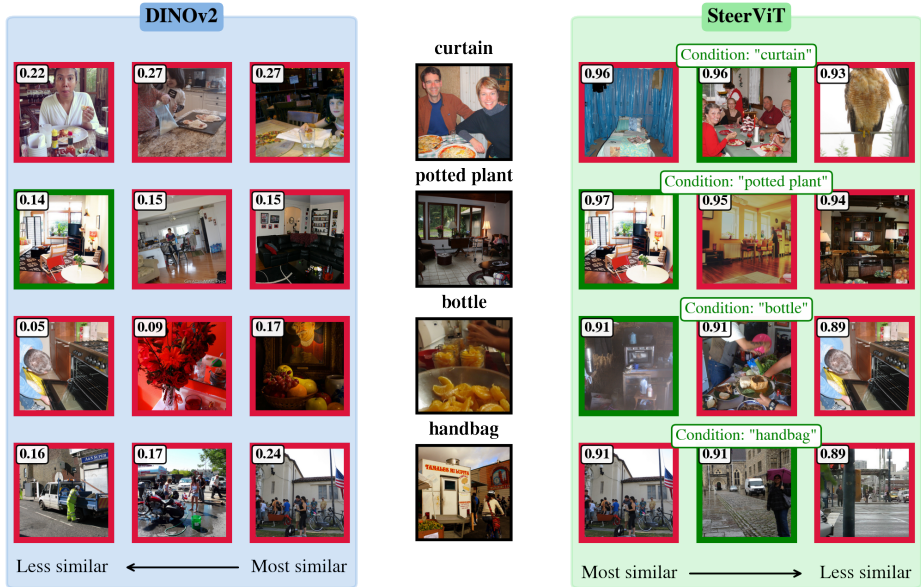
Fig. 13: Qualitative image retrieval results on the GeneCIS Focus Object split. Green / red border indicates whether images contain the object of interest and match the scene context of the query. DINOv2 is biased towards scene similarities whereas SteerViT additionally considers the presence of the target object.
