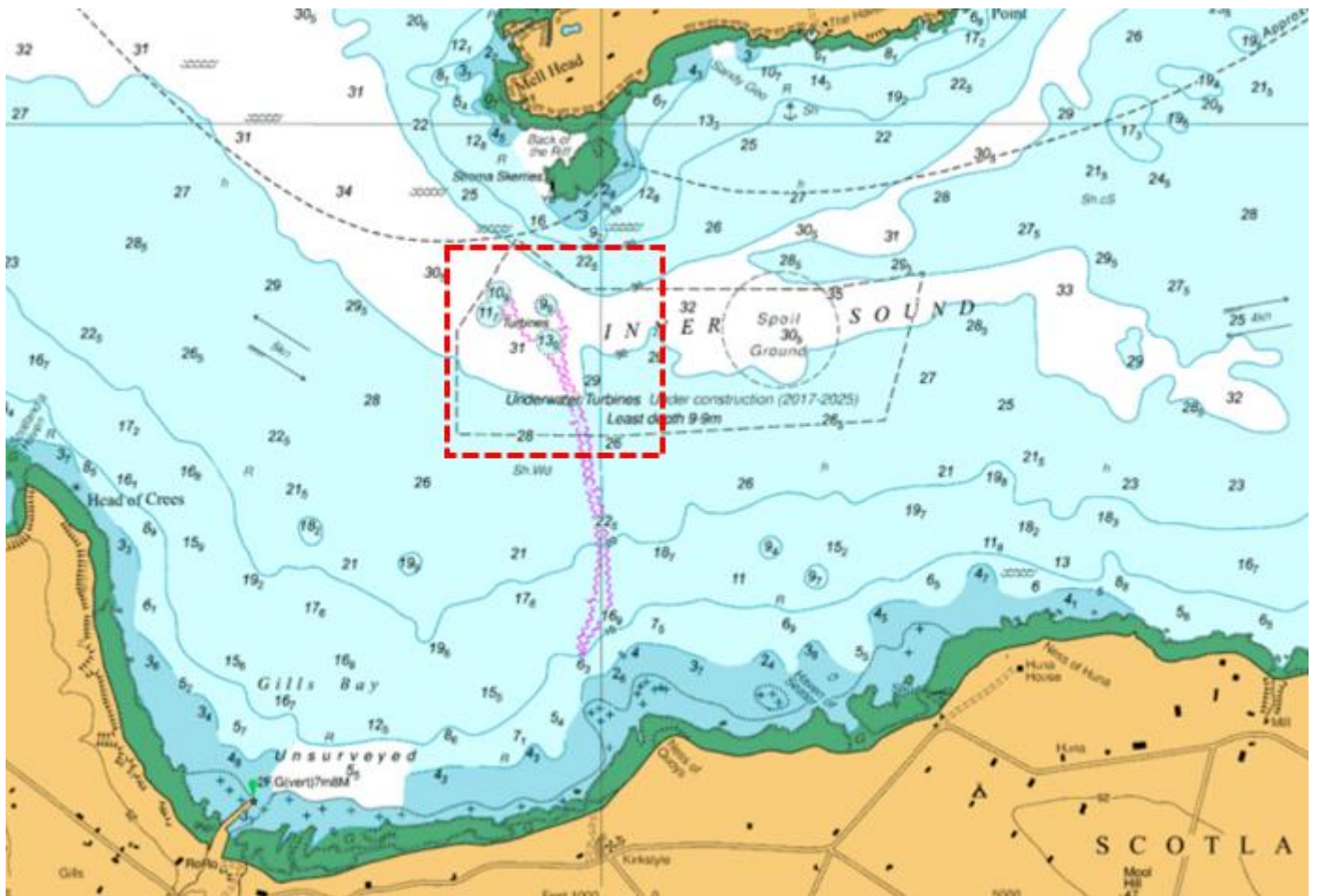
Figure 2 – Chart 2851 © UKHO
