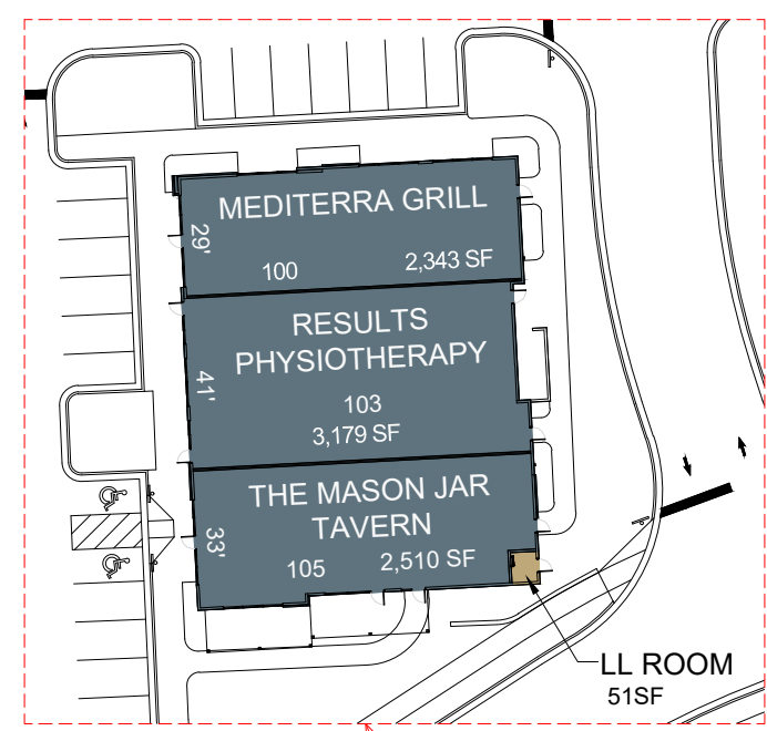
RETAIL "A" Scale 1"= 50'
