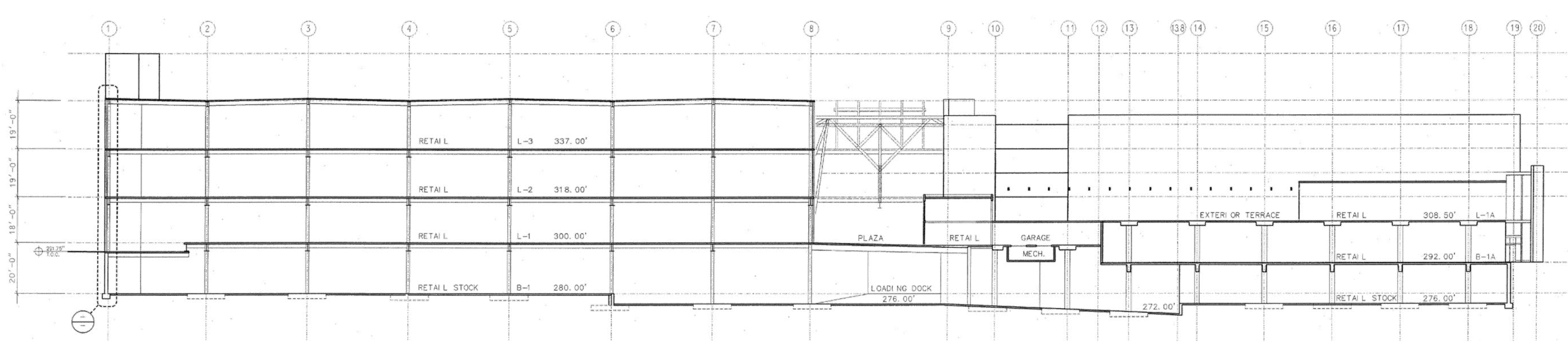
LEVEL 5
