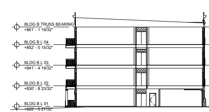
NORTH-SOUTH BUILDING SECTION
