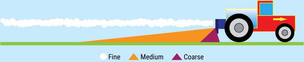
Source: GRDC Weather Essentials for Pesticide Application Booklet, 2017; author: Graeme Tepper.
