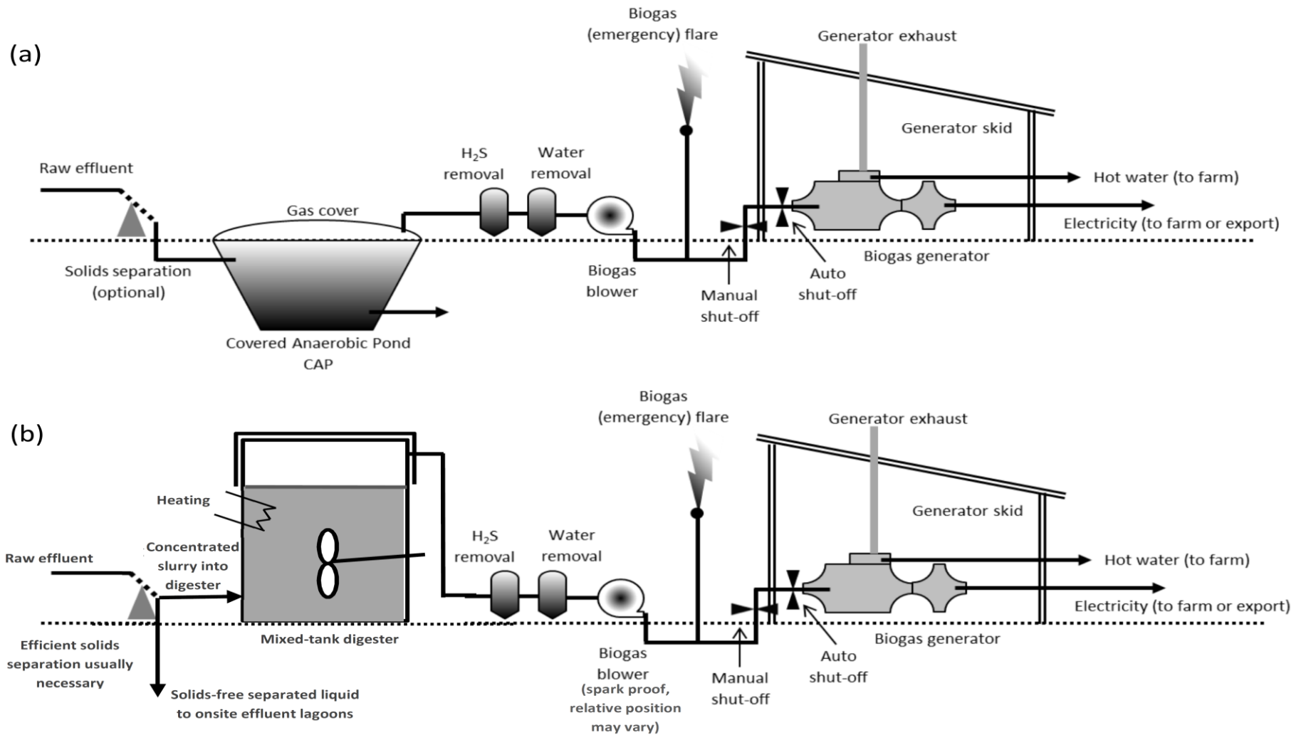
Figure 1.1 Typical components of a piggery biogas plant with a (a) covered anaerobic lagoon or (b) an above-ground mixed tank digester
