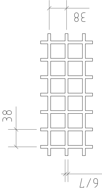
Plan view
