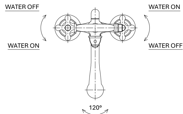
ROTATION ANGLE OF THE WATER OUTLET
