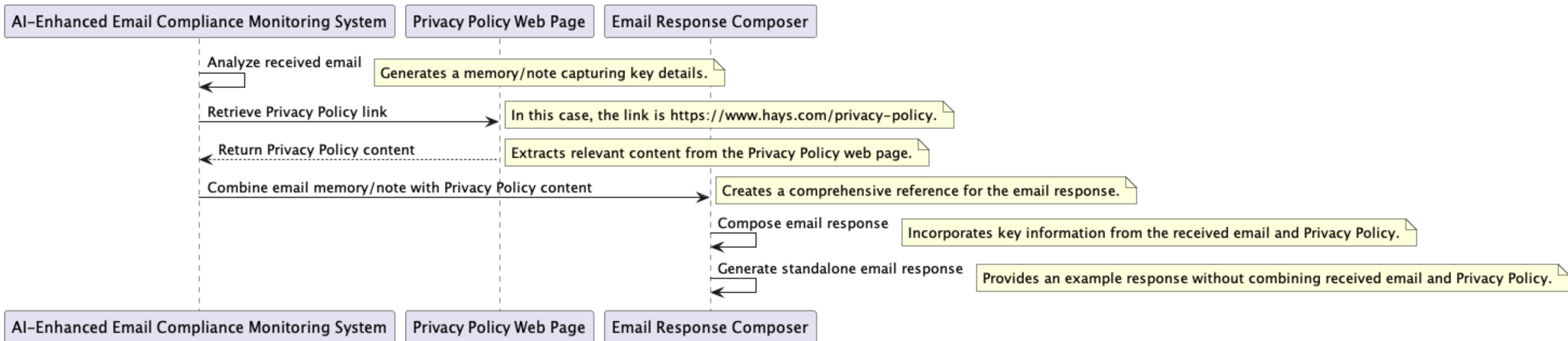
AITOversight: AI-Enhanced Email Compliance Monitoring System Pipeline
