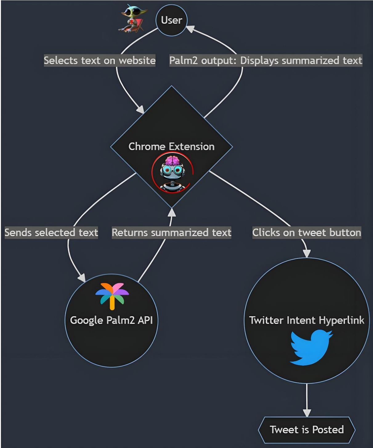
Figure 1: Application workflow
