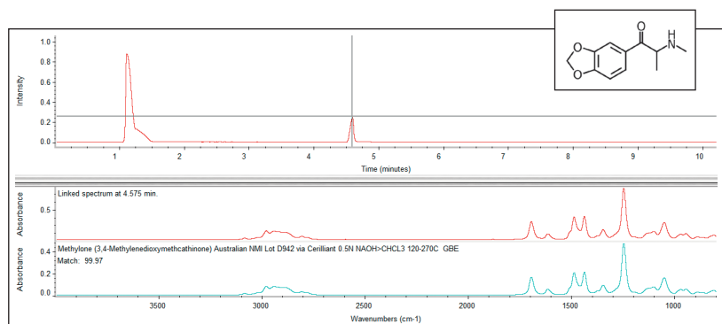
Figure 9: Output from the OMNIC Mercury GC analysis of the entire GS profile for a methylene sample. This bath salt sample was run using a longer (30 meter) column.
