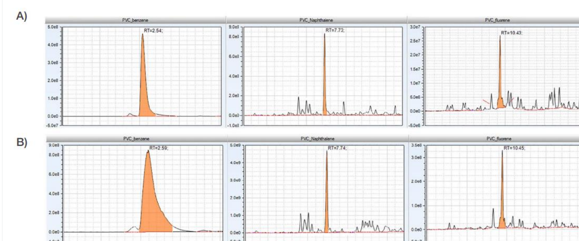
Figure 4. Identification of PVC, A) standard and B) stormwater sample.
