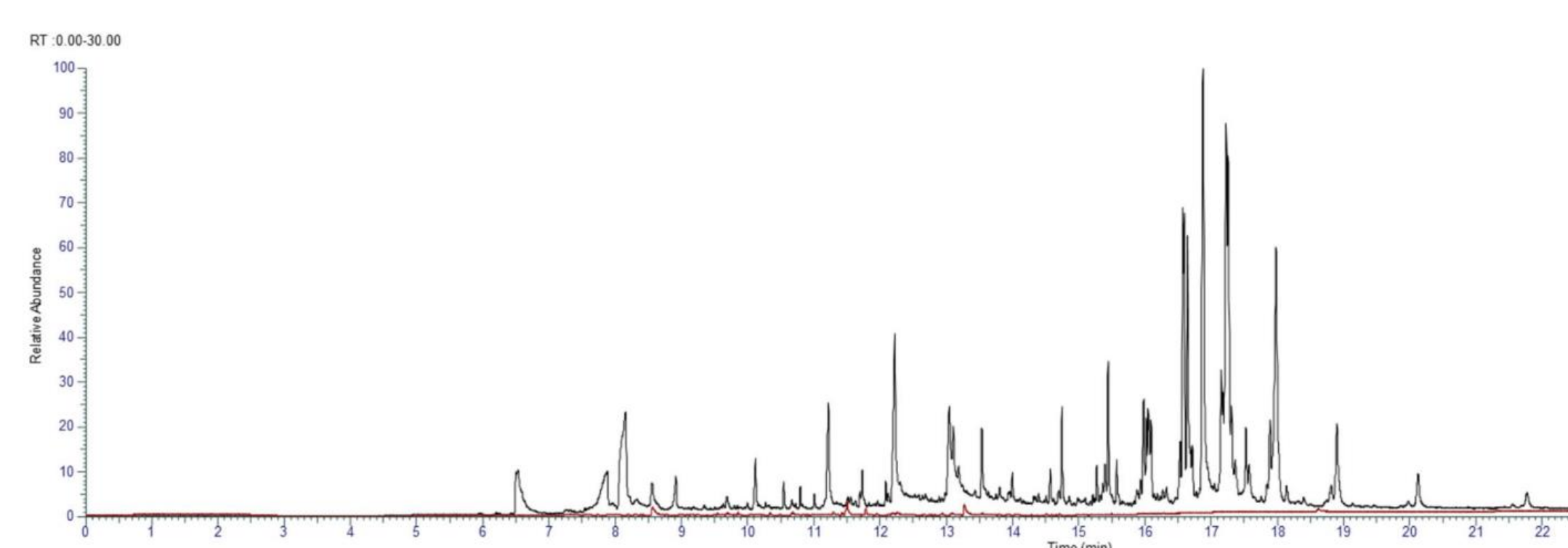
Figure 2. Total ion current chromatogram (m/z 40–600) obtained for a milk sample (black chromatogram) compared with a solvent standard of a mix of polymers (red chromatogram) after the TD step.
