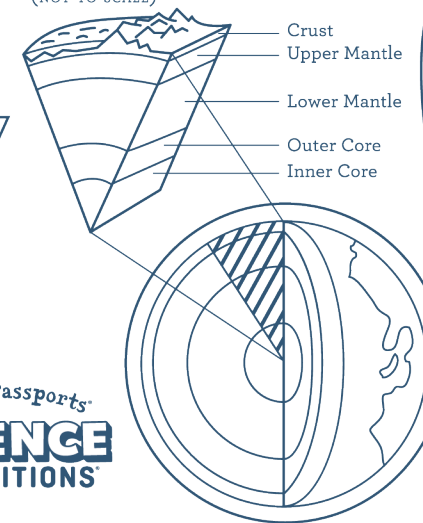
fig. 9 Earth Cross-Section (NOT TO SCALE)
