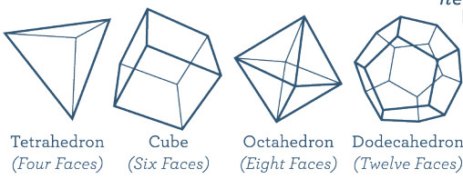
fig. 4 Crystal Shapes
