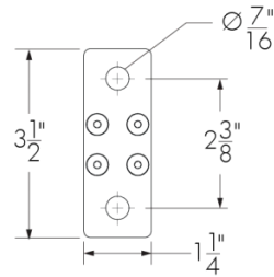
WAMN28 - Mounting Hole Pattern
