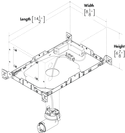
REVO SPOT SEMI-RECESSED Medium Wallwash (RS)
