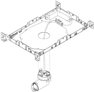
REVO SPOT SEMI-RECESSED Medium Wallwash (RS)
