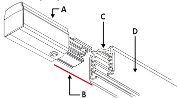
Lumencore Track Double Circuit System and Live End Feed (Left)
