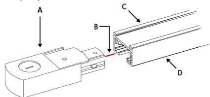
Lumencore Track Single Circuit System and Live End Feed (Left)
