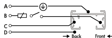
One Circuit Wiring Detail - Track
