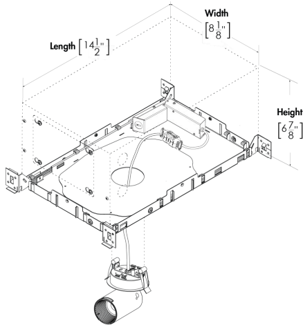
REVO SPOT SEMI-RECESSED Medium (RS for NS, ENS, S, NF, FL, WFL and EWFL Optics)
