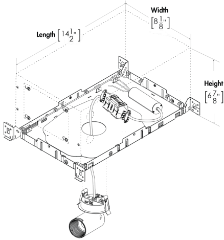
REVO SPOT SEMI-RECESSED Medium (RS for VN Optic)
