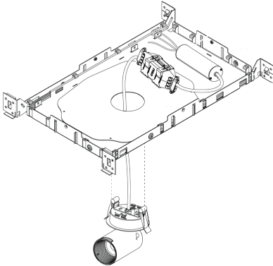
REVO SPOT SEMI-RECESSED Medium (RS for VN Optic)
