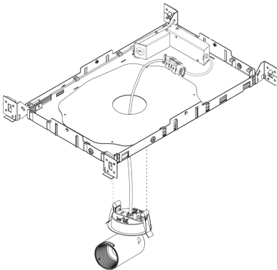
REVO SPOT SEMI-RECESSED Medium (RS for NS, ENS, S, NF, FL, WFL and EWFL Optics)
