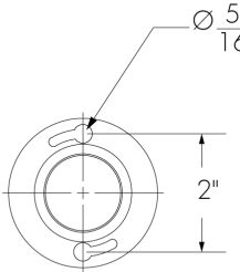
Mounting base screw hole pattern
