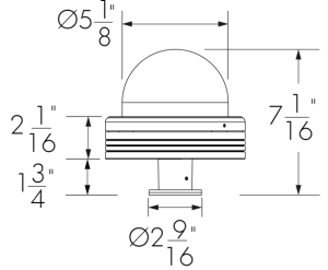
Front view Dome lens shown
