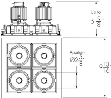
Ceiling cutout: 9 1/4" x 9 1/4" Maximum ceiling thickness: 1"
