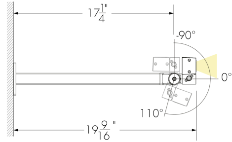
Under-mount installation
