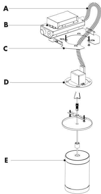
Exploded view
