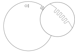
Diffuser Lens 5 (5 Notches)
