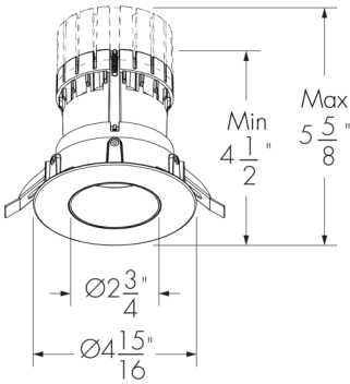
Round trim (Shown with 1 in in ceiling springs) Round trim ceiling cutout: Ø4.5 in
