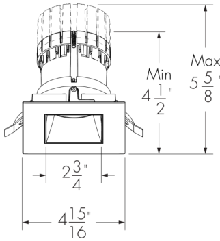
Square trim (Shown with 1 in in ceiling springs) Square trim ceiling cutout: 4.5 in x 4.5 in
