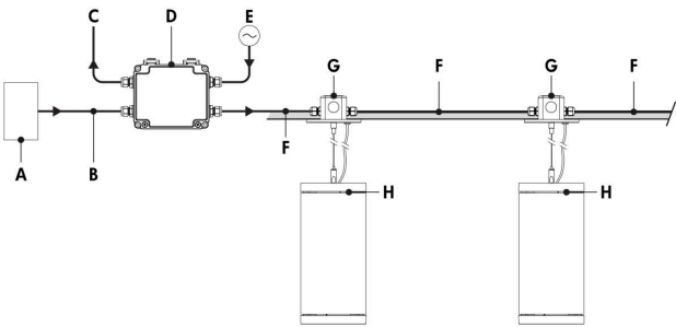
Daisy Chain Layout (DMX/RDM)
