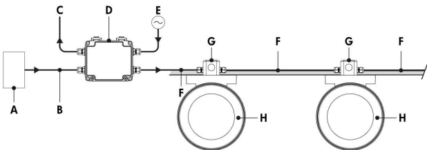
Daisy Chain Layout (DMX/RDM)
