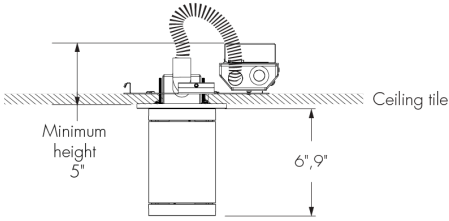
Ceiling cutout: Ø 4 " Maximum ceiling thickness: 1 3/4"
