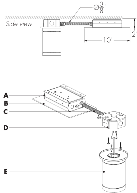
Exploded view
