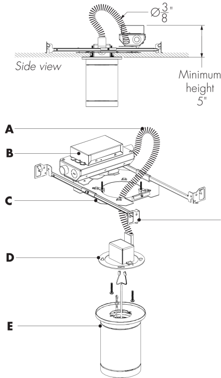
Exploded view
