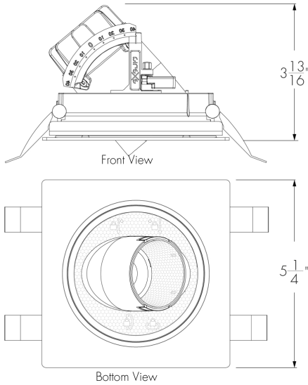
DT1S Housing With Trim
