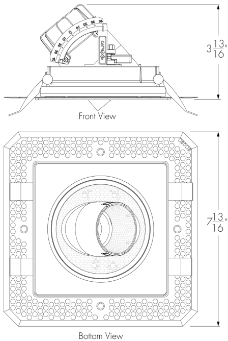
DT1S Housing Trimless
