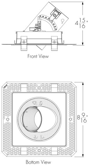
DT1S Housing Trimless
