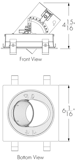
DT1S Housing With Trim
