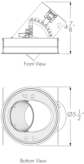
DT1R Housing With Trim and Trimless
