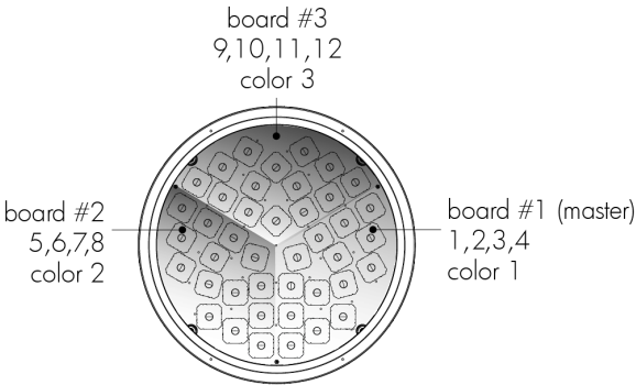
MRGBA, MRGBWP and MRGROYWP color mixing options
