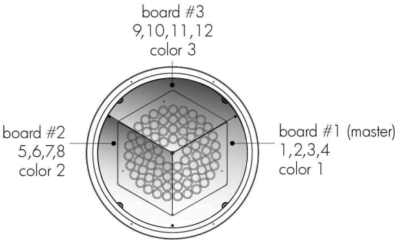
RGBW30K, RGBW40K and RGBA color mixing options
