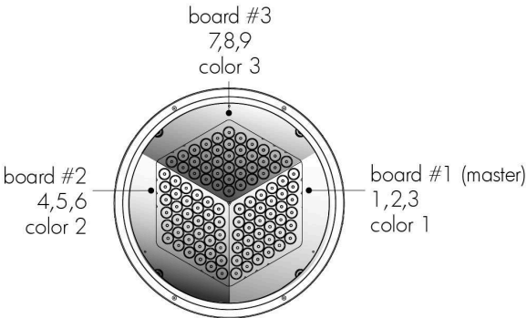
RGB color mixing option
