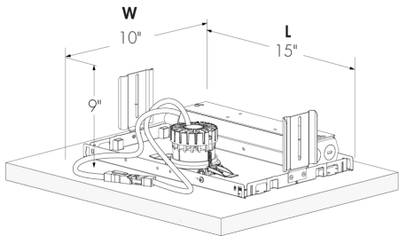
Ceiling Cavity Space Requirements for Fixtures With Trim
