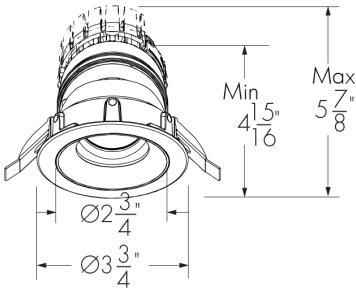
Round trim (Shown with 1 in ceiling springs) Round trim ceiling cutout: Ø3.25 in
