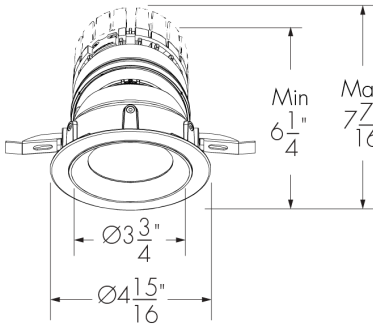
Round trim (Shown with 1 in ceiling springs) Round trim ceiling cutout: Ø4.5 in
