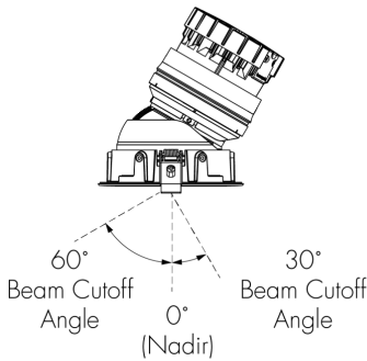
Side view (Based on 30° fixed tilt)
