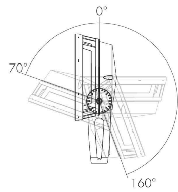
Standard yoke
