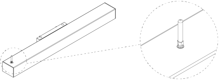
Fixture With Button Type Photocell Option
