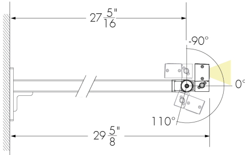
Under-mount installation
