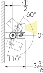
Under-mount installation
