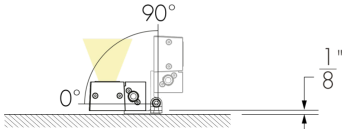
Under-mount installation
