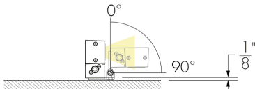
Side-mount installation
