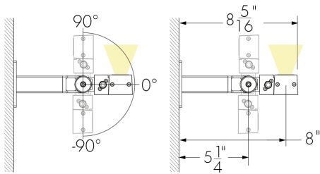
Side-mount installation
