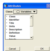
Attributes Dialog
