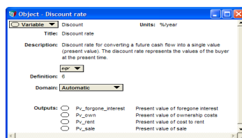
Object Window
