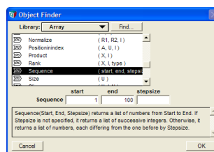
Object Finder
