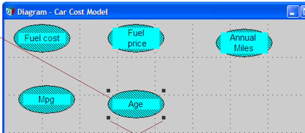
Handles
