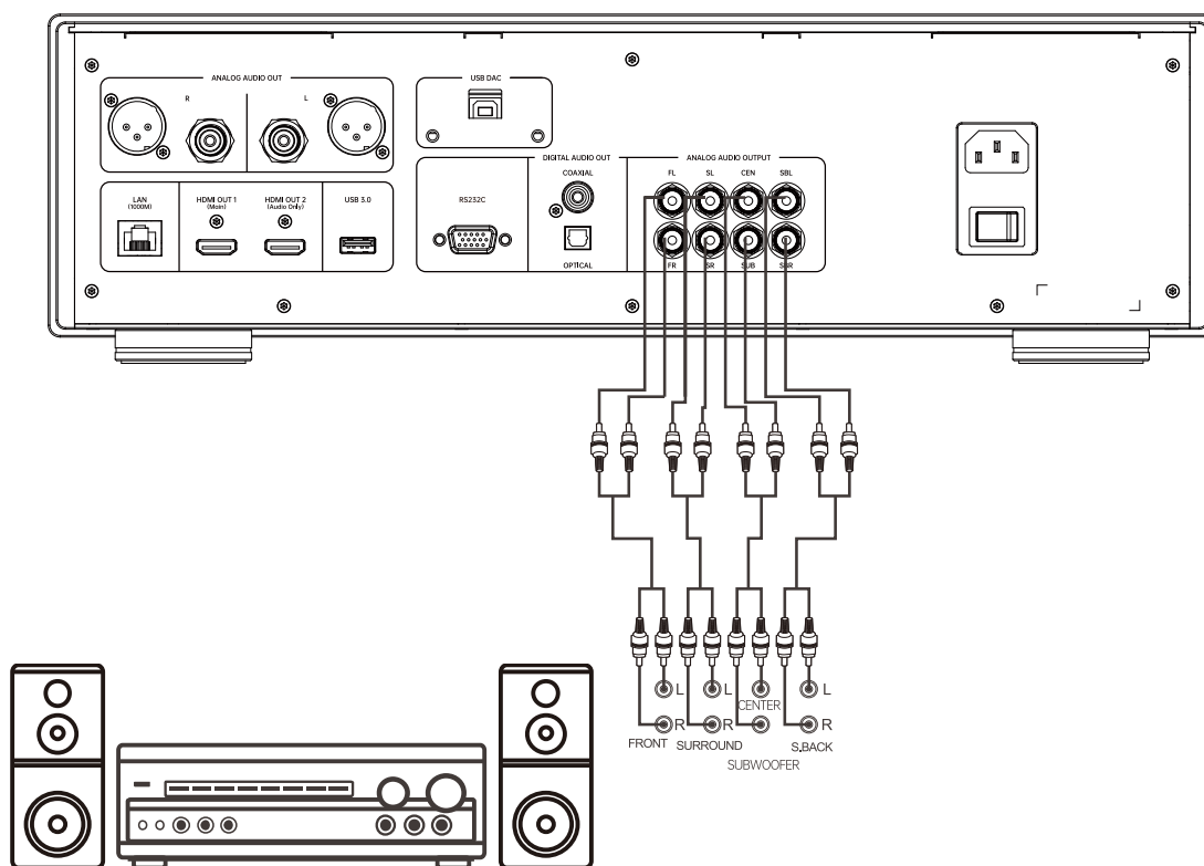
Receiver/Amplifier with 7.1ch Audio Input
