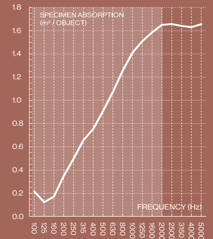
Sound Absorption Results – Lumenwerx Mikro Wafer 2 rows of 4 units spaced 49" o.c, bottom edge of unit 48" from the floor.
