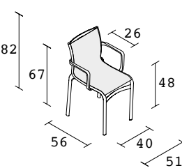
Highframe 40 armrest outdoor / 417_O
