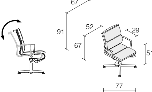
Meetingframe 52 armrest soft / 484
