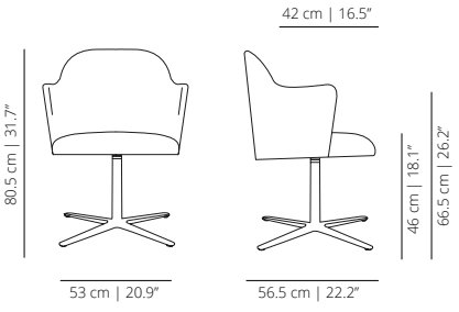
ALSIPLABR flat swivel base chair with arms
