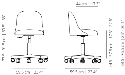
ALSIBR caster base chair
