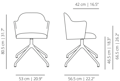
ALSIMABR pyramid swivel chair with arms
