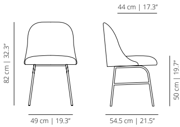
ALSIMÉ metal base chair
