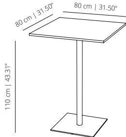
ST110C80_ table 80x80 | table 31 1/2 x 3 1/2
