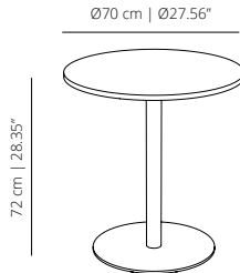
ST72D70_ table round 70 | table round 27 61/64
