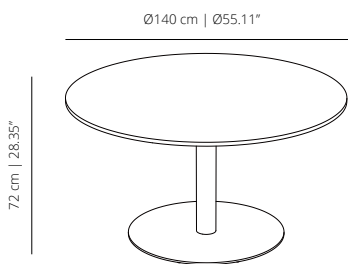
ST72D140_ table round 140 | table 55 1/8
