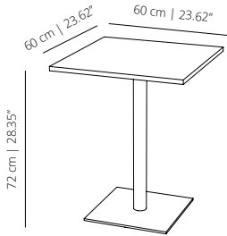
ST72C60_ table 60x60 | table 23 3/8 x 23 3/8
