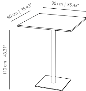
ST110C90_ table 90x90 | table 35 7/16 x 35 7/16
