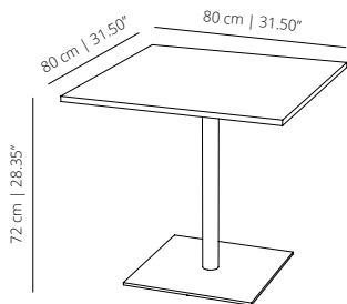
ST72C80_ table 80x80 | table 31 1/2 x 31 1/2
