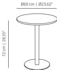
ST72D60_ table round 60 | table round 23 3/8
