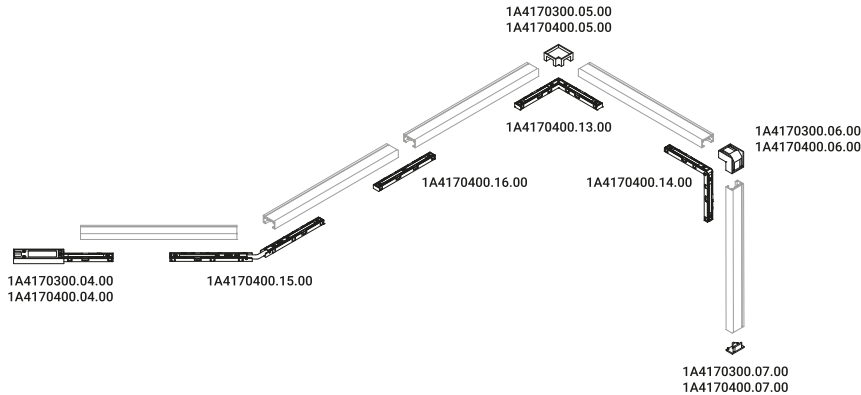
Layout example of wall and ceiling version
