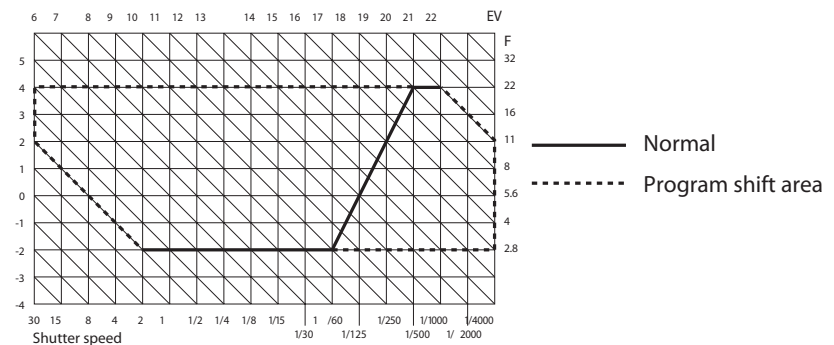
Phase One 645 program shift chart
