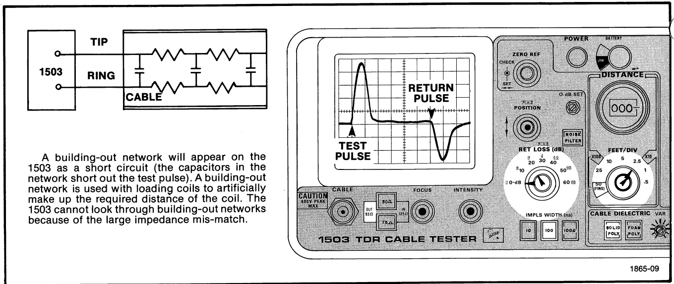
Fig. 2-10. Building-out network.
