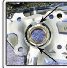
Inspect camplate for scoring, if scoring is present replace camplate. Scoring will effect oil psi & oil scavenging
