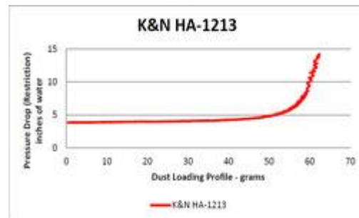
Flow Chart for K&N 2013 Honda PCX 150 and 2013 and 2014 Honda PCX 125 Air Filter HA-1213
