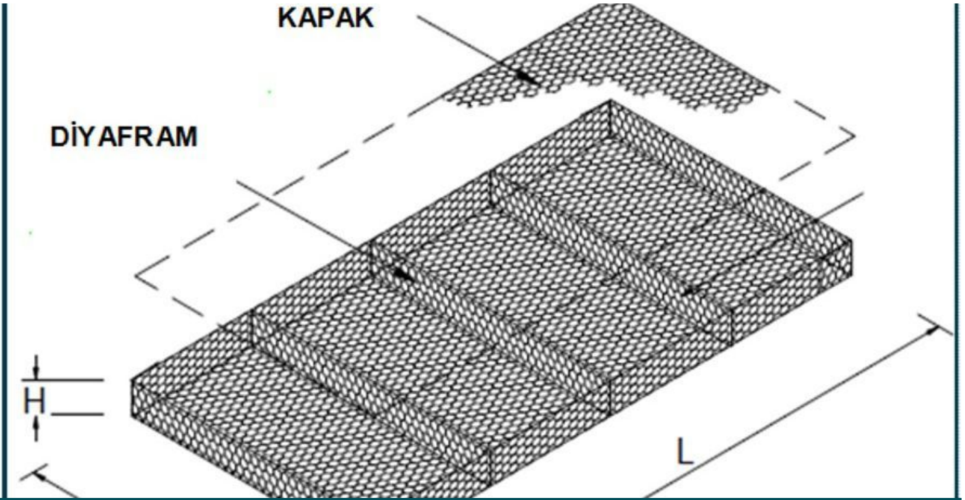
Mattress Gabion Structure
